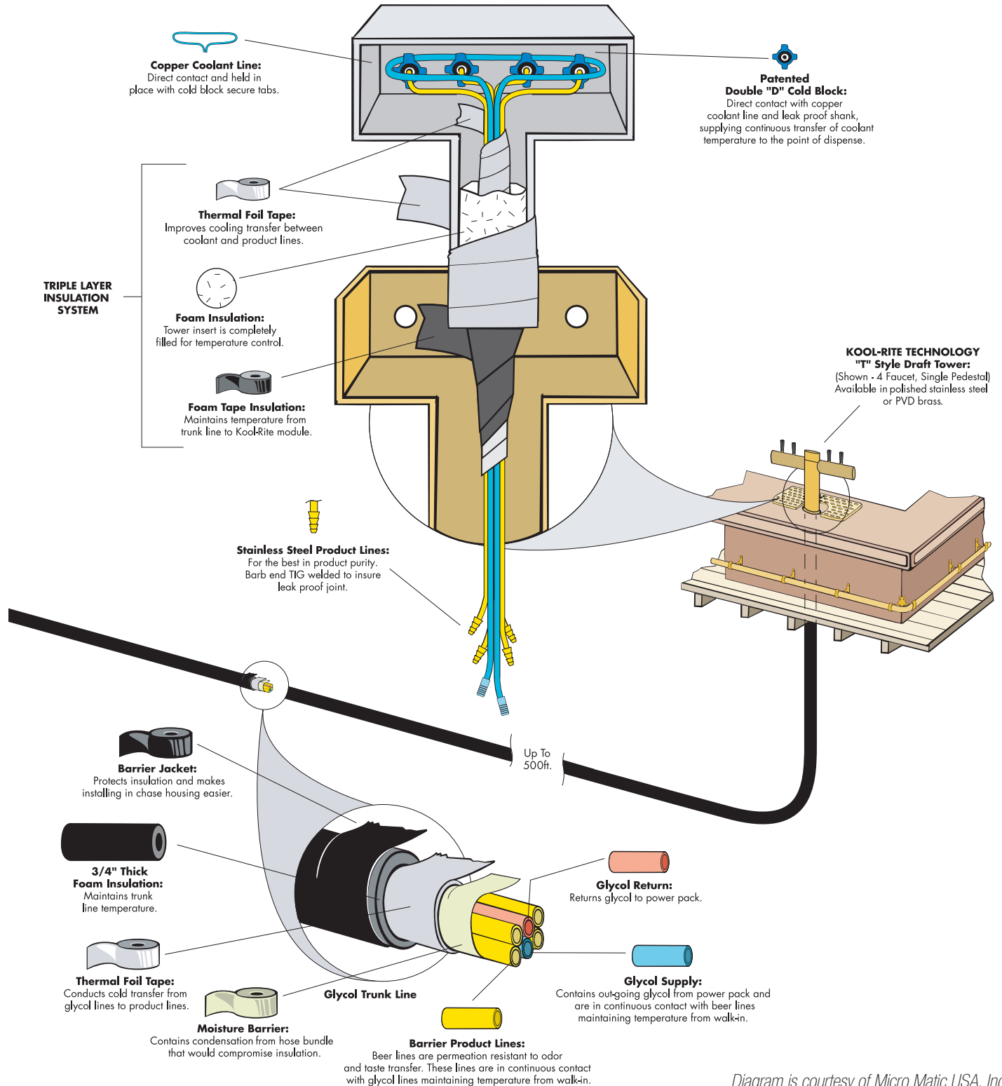
Cut-Away View KOOL-RITE TECHNOLOGY Drop-In Module Fabrication
